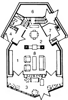
9 Plan view - ground floor
